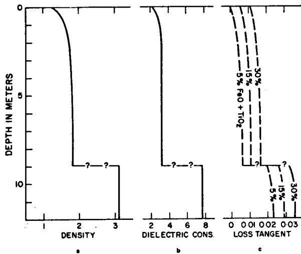
Figure 3.—(a) An equation for density as a function of depth in the lunar soil given as Z = 0.01(-1 + \sum A_i e^{iZ}) . (b) The dielectric constant as a function of depth for the density profile of (a). The sharp change between soil and rock illustrated by —? —? —? occurs at an unknown depth. (c) The loss tangent as a function of depth for the density profile of (a). The three curves correspond to 5-, 15-, and 30-percent FeO + TiO 2 .
