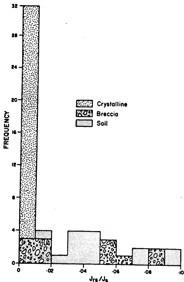
Figure 10.—Histogram of values of J_{rs}/J_s for different types of lunar samples. Small values of this quantity imply multidomain materials which are magnetically soft. ( J_{rs} = saturation remanence; J_s = saturation magnetization.)
