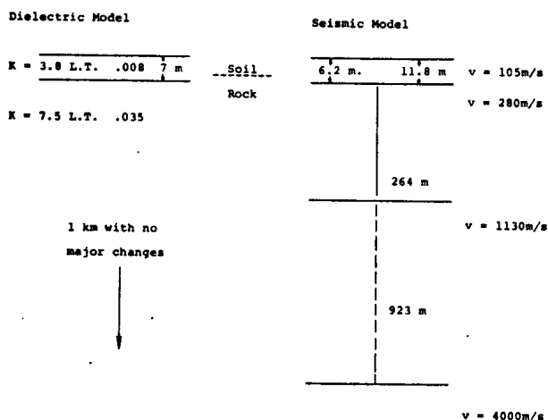
Figure 6.—Cross section at the Taurus-Littrow landing site determined from the surface electrical properties experiment and from the lunar seismic profiling experiment.
